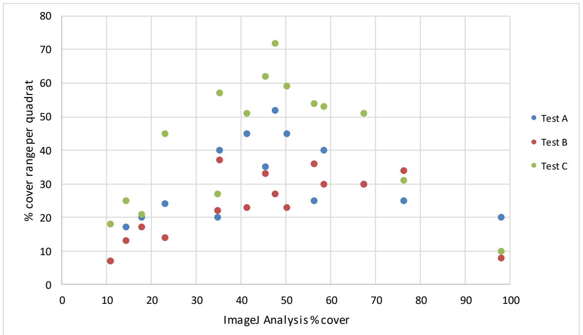
Figure 1: Scatter graph showing the range of % cover results per quadrat across all three test methods for opportunist macroalgae.
