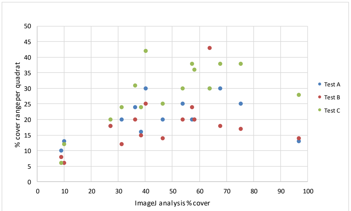
Figure 1: Scatter graph showing the range of % cover results per quadrat across all three test methods for opportunist macroalgae.
