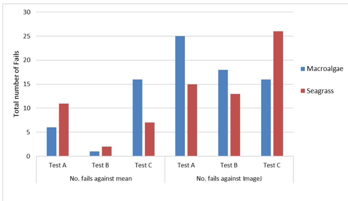
Figure 3: Number of Fails recorded across all tests for macroalgae and seagrass quadrats for OMC RT12.
