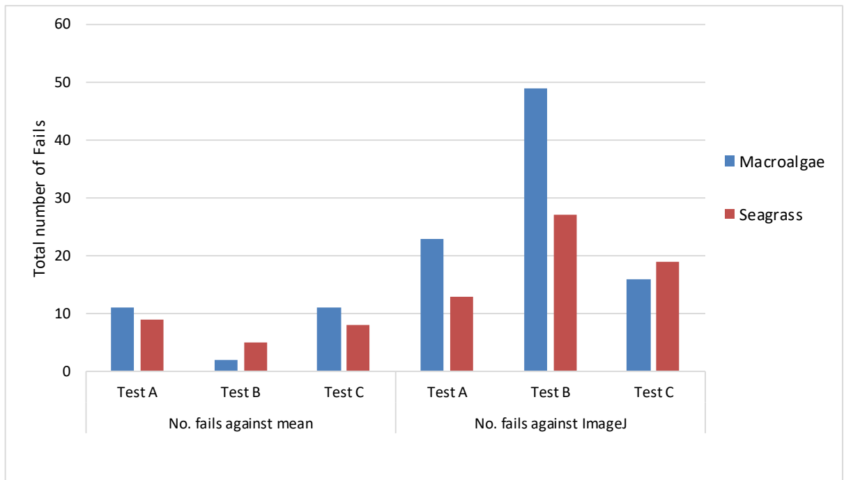
Figure 4: Number of Fails recorded across all tests for macroalgae and seagrass quadrats for OMC RT11.
